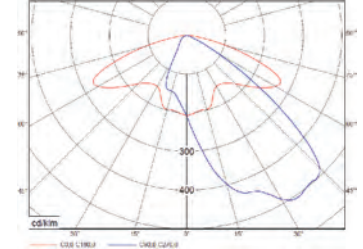
Asymmetric, LS, 8700lm
