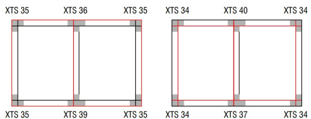
Floor view
